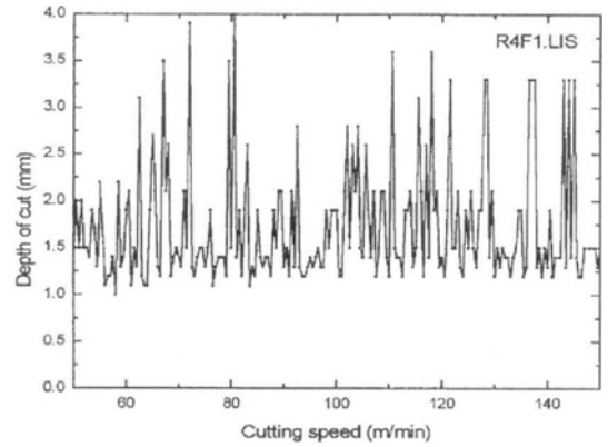
Fig. 13 Unstable borderline for nose radius 0.4 mm, feed 0.1 mm/rev
