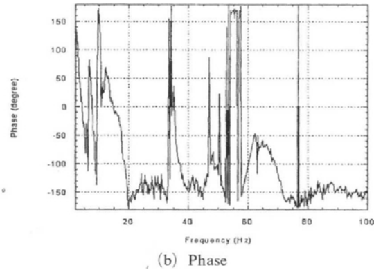
Fig. 6 Frequency response functions between a tool and a steel workpiece
