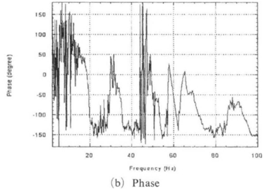
Fig. 5 Frequency response functions between a tool and an aluminium workpiece
