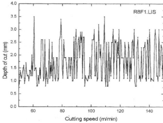
Fig. 10 Unstable borderline for nose radius 0.8 mm, feed 0.1 mm/rev
