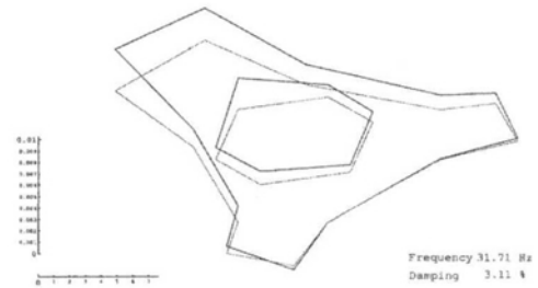
(b) Mode shape at 31.7 Hz
