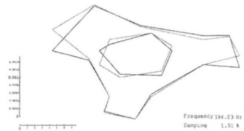
(e) Mode shape at 194 Hz
