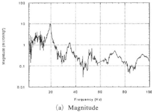
Fig. 5 Frequency response functions between a tool and an aluminium workpiece
