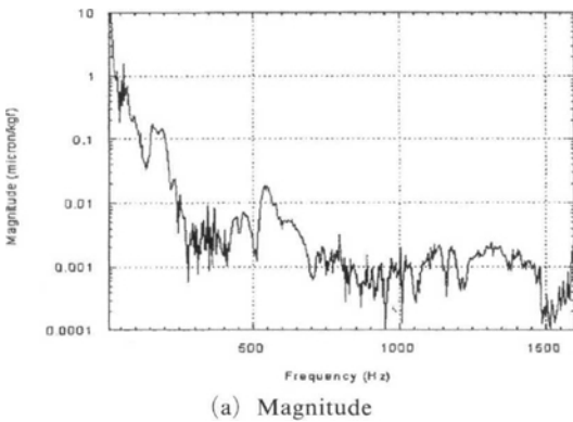
Fig. 7 Frequency response functions between a tool and a steel workpiece shown in broad frequency range
