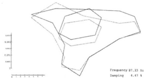
(c) Mode shape at 87.3 Hz
