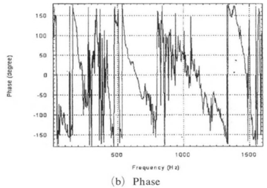
Fig. 7 Frequency response functions between a tool and a steel workpiece shown in broad frequency range
