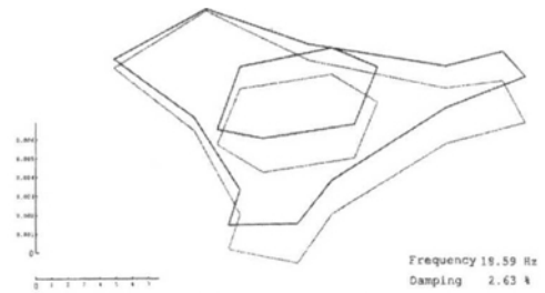
(a) Mode shape at 18.6 Hz
