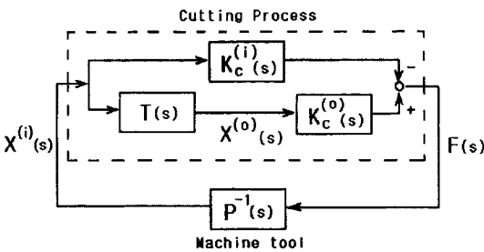
Fig. 8 A block diagram for the chatter loop
