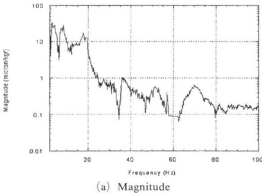
Fig. 6 Frequency response functions between a tool and a steel workpiece
